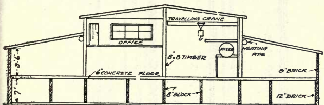
SECTIONAL ELEVATION C. D.
